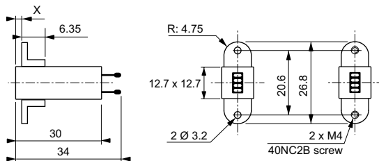
CM5207 / CM5207T
