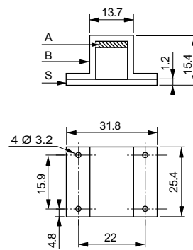
Mounting clip BR001
