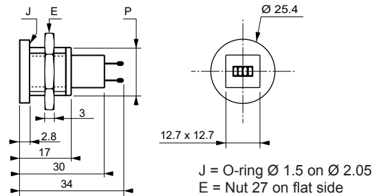
CM5205 - Tightening torque : 5 Nm
