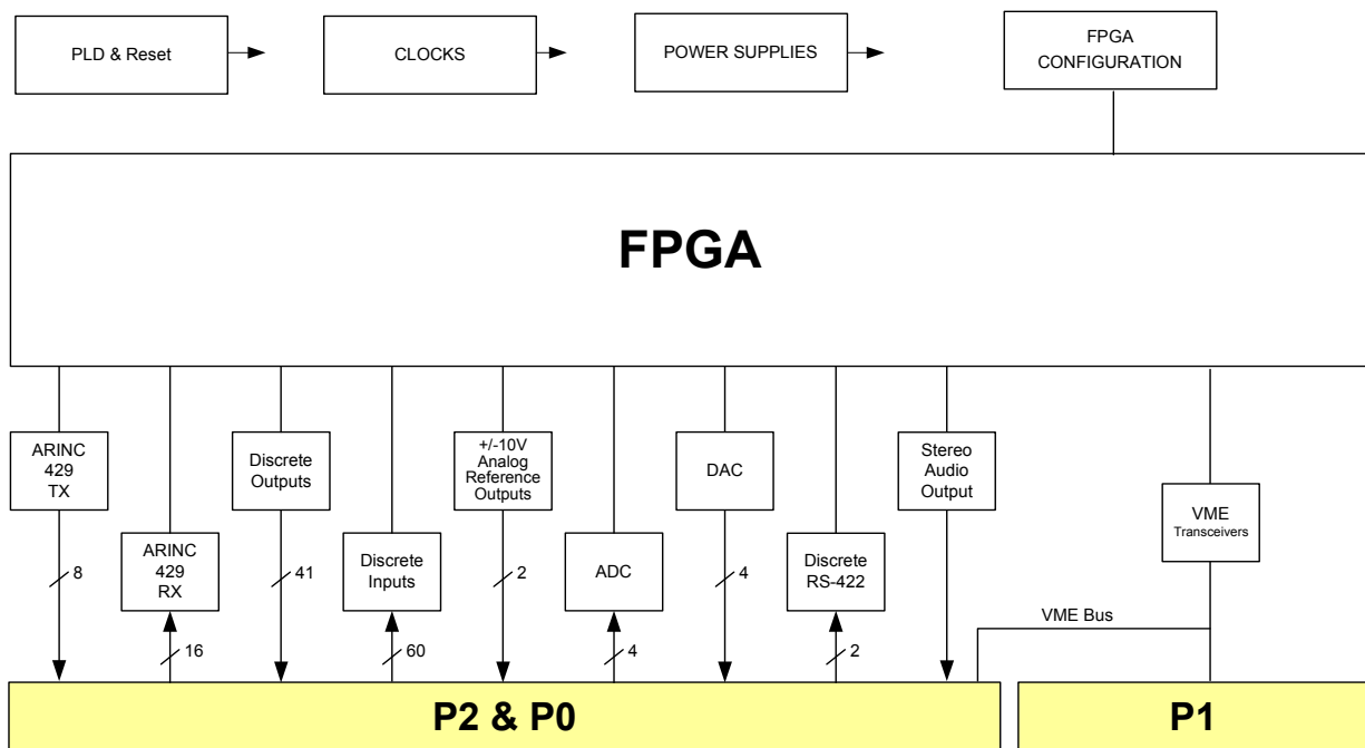
C437 Block Diagram
